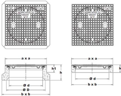
type N 352 NB-R Centerfix 170 - 240 mm
